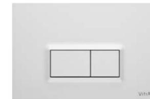
Loop R Mechanical flush plate Gloss White £51 - 740-0600 Matt Black £44 - 740-0611 Chrome Plated £51 - 740-0680 Matt Chrome Plated £56 - 740-0685 Anti-fingerprint £85 - 740-0686 Compatible with all VitrA wall-hung 760-frames, 748-frames and 742-frames H: 165mm W: 244mm P: 8mm
