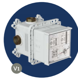
V-Box concealed shower valve £92 - A42263 H: 146mm P: 77-142mm
